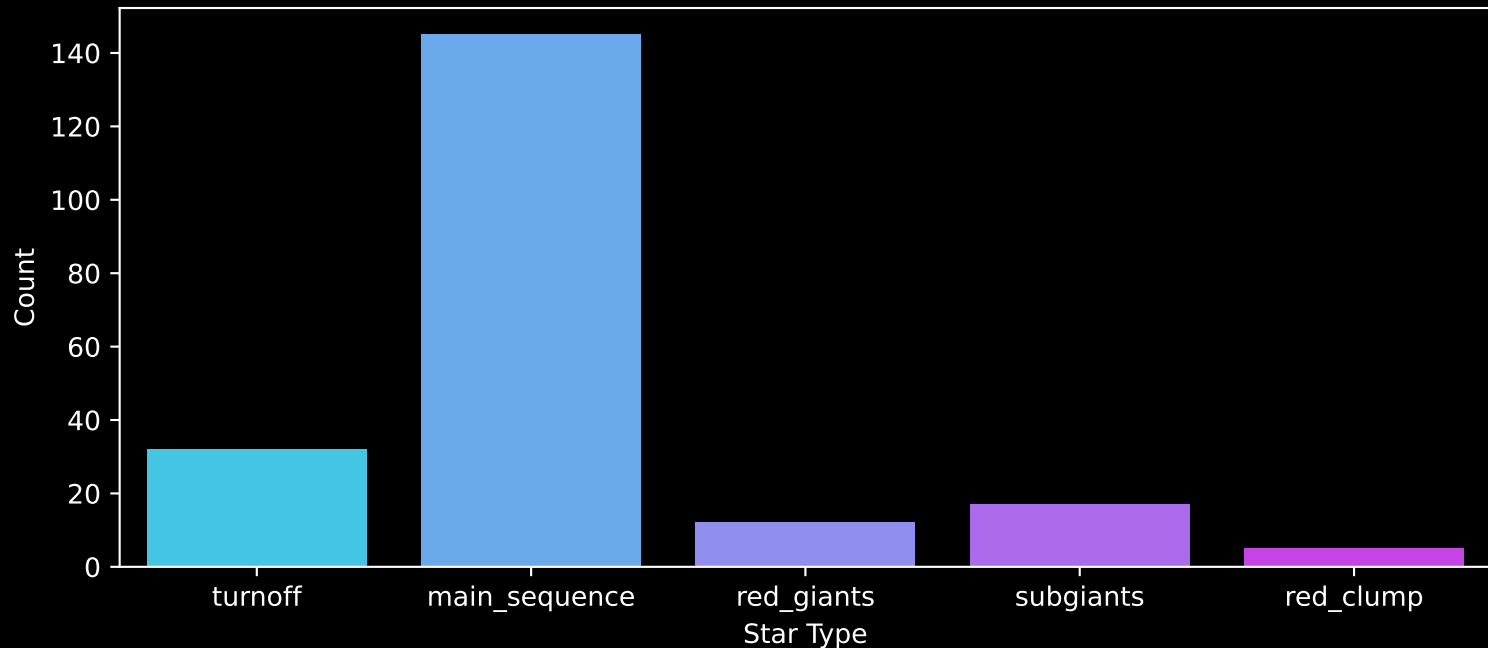
APOGEE DR17 Field: [120-61-O] Count plot of Star Type
