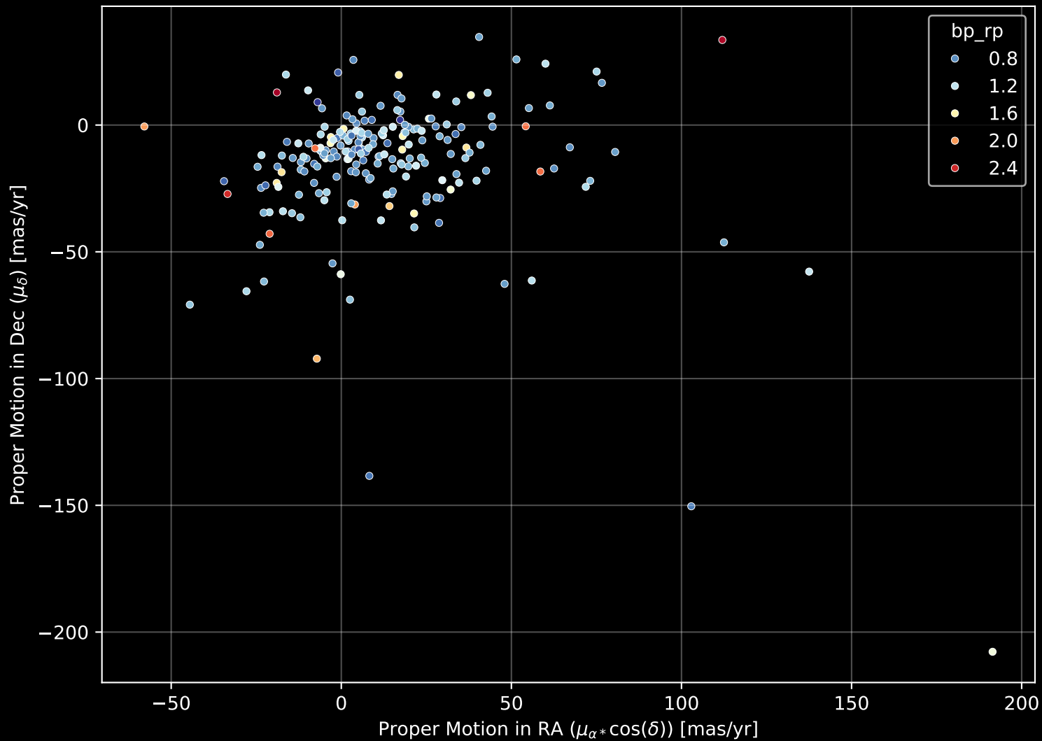
APOGEE DR17 Field: [120-61-O] Proper Motion Diagram (n= 211)
