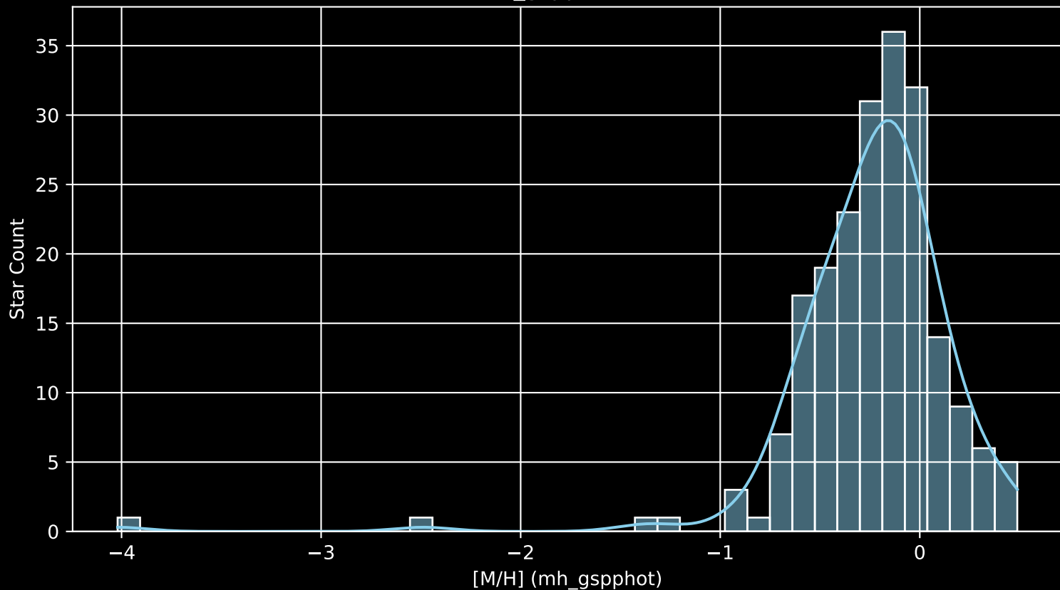
APOGEE DR17 Field: [120-61-O [M/H] (mh_gspphot) (n= 207)
