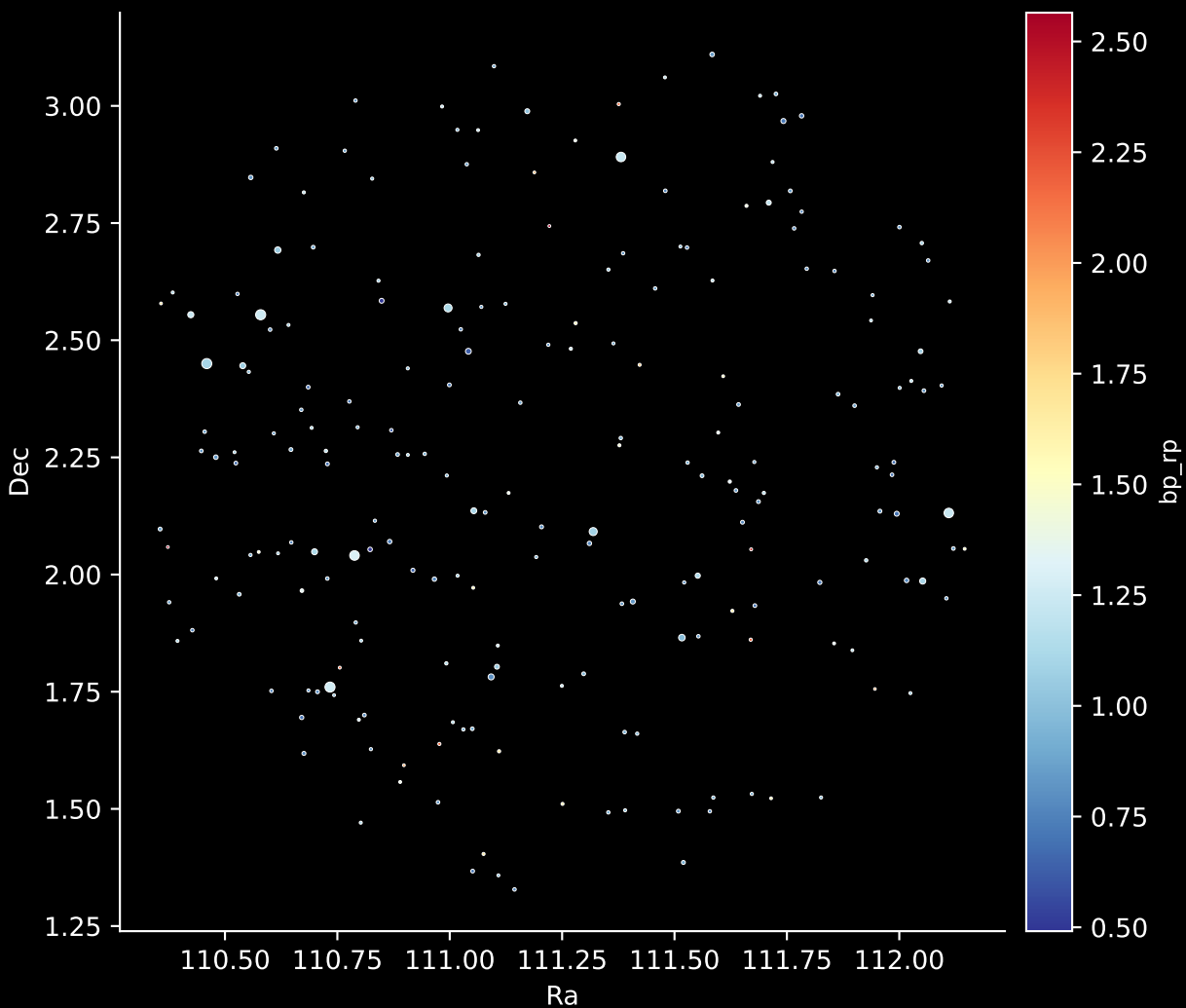
APOGEE DR17 Field: [120-61-O] Stars: 211
