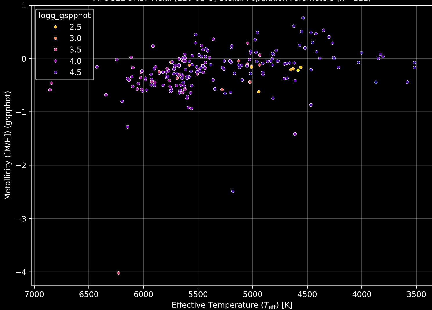
APOGEE DR17 Field: [120-61-O] Stellar Population Parameters (n= 211)
