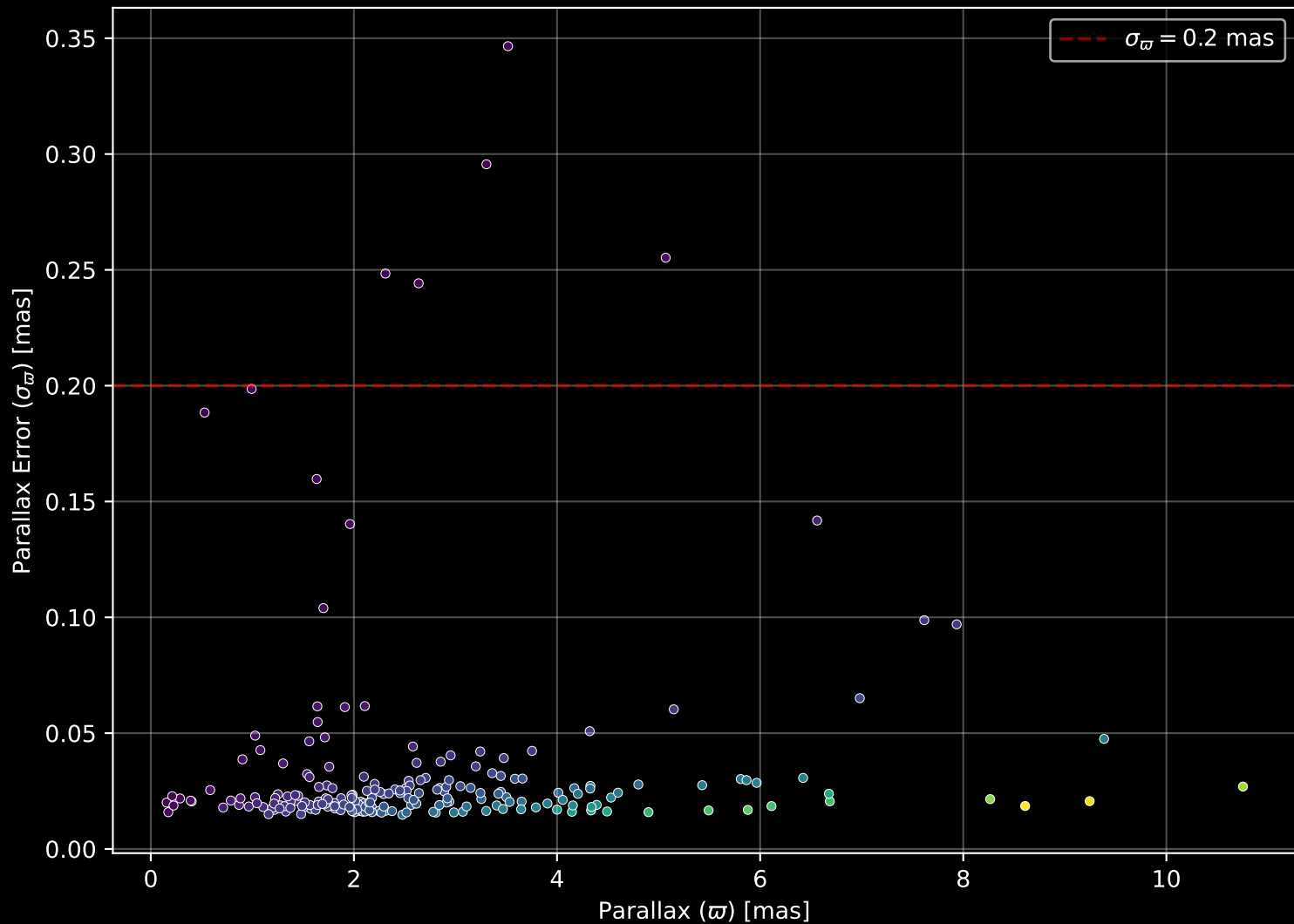
APOGEE DR17 Field: [120-61-O] Parallax Quality (n= 211)
