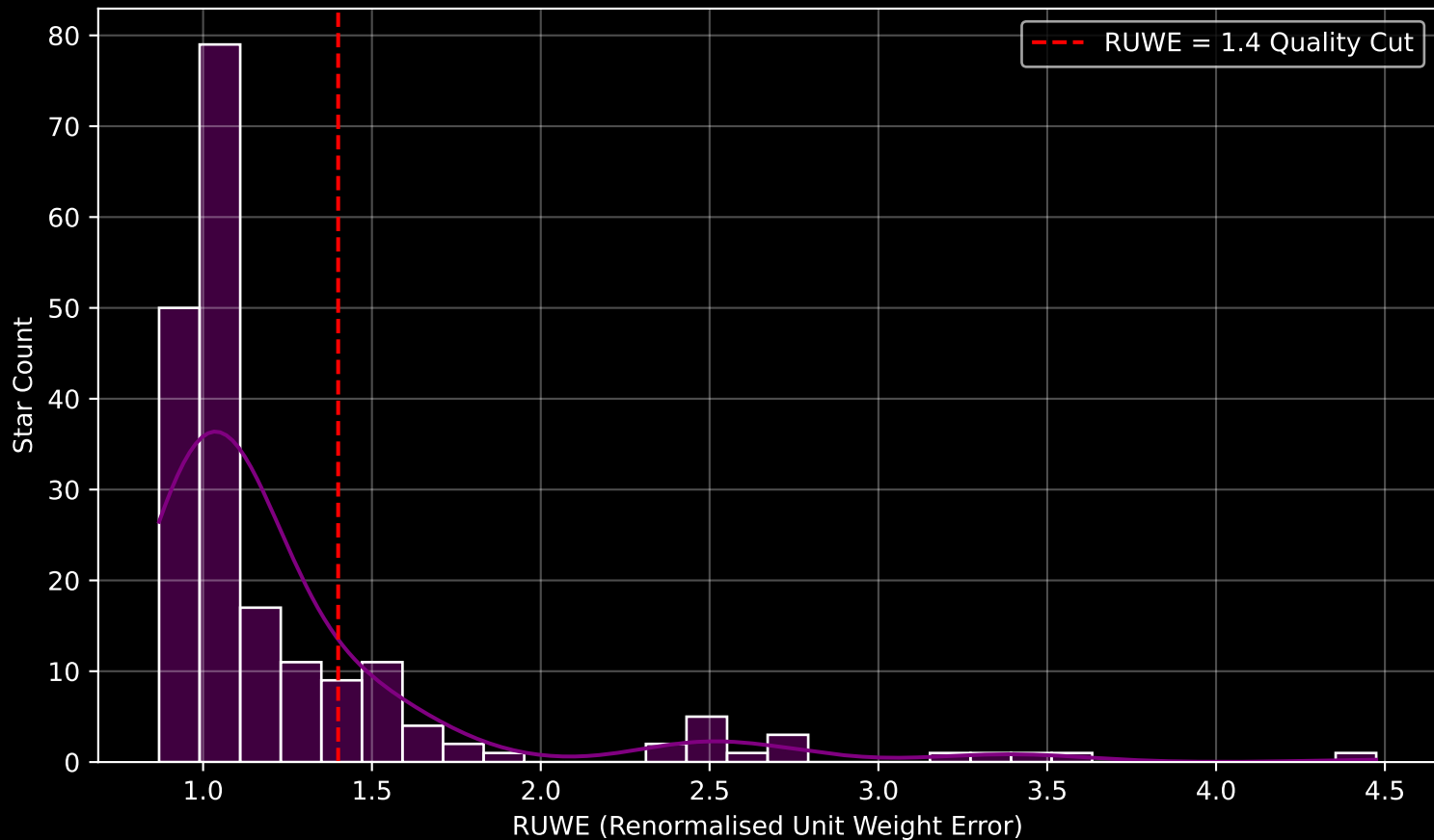
GAPOGEE DR17 Field [120-61-O] RUWE Distribution (n= 200)
